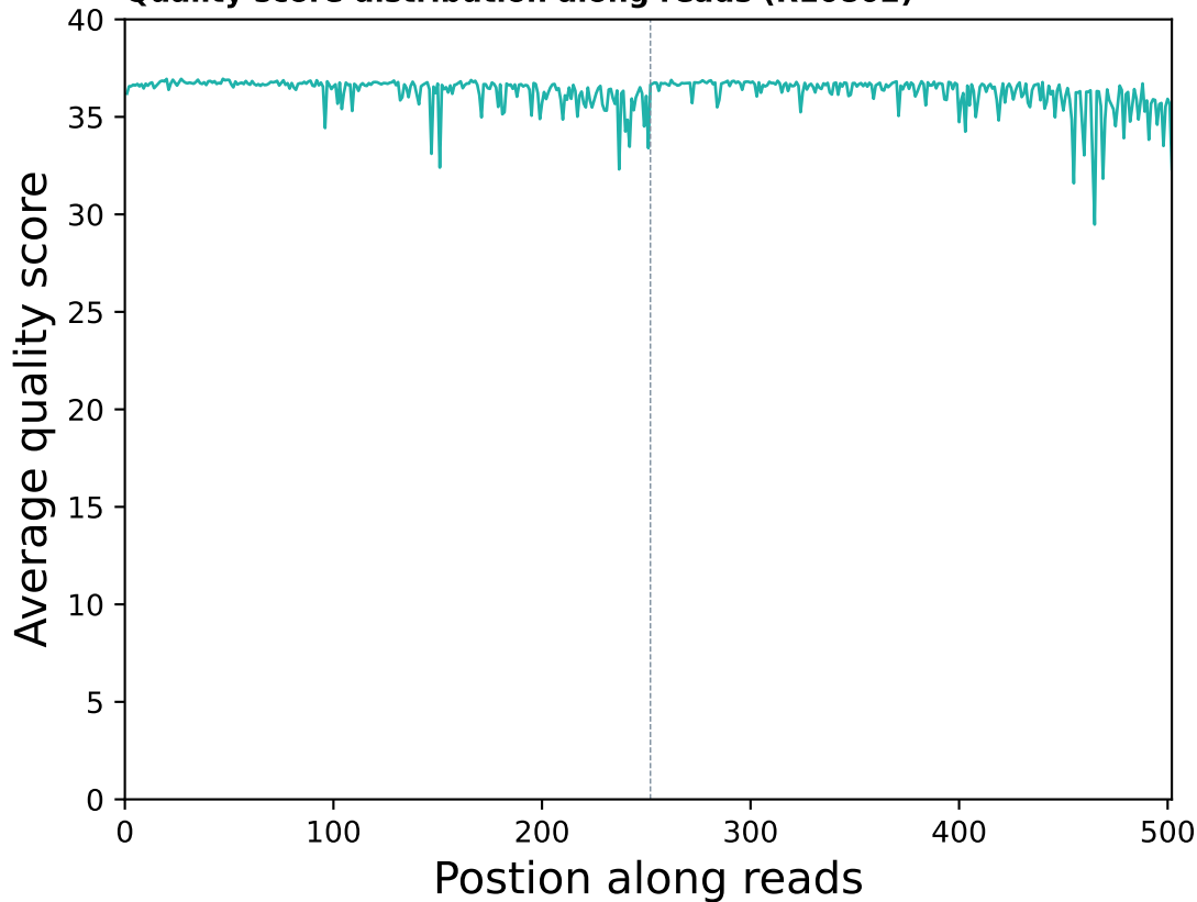
Quality score distribution along reads (R10802)
